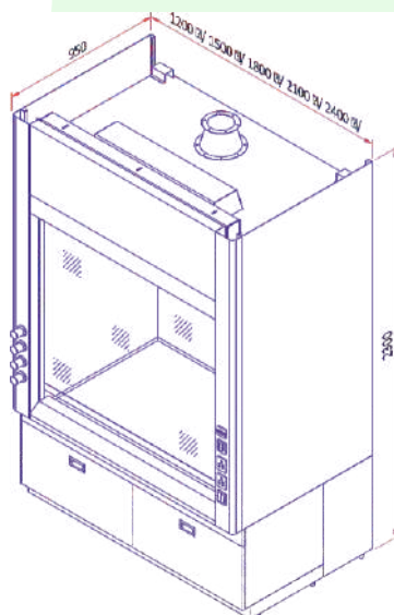
Low Bench Fume Hood
