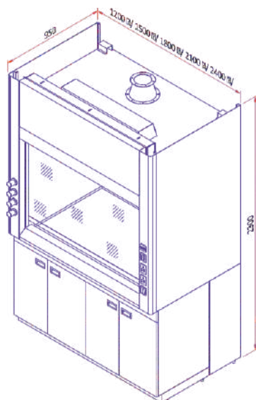
STD Bench Top Fume Hood
