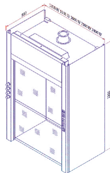
Walk-in Fume Hood
